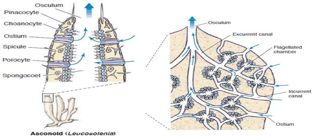
Asconoid ( Leucosolenia )
